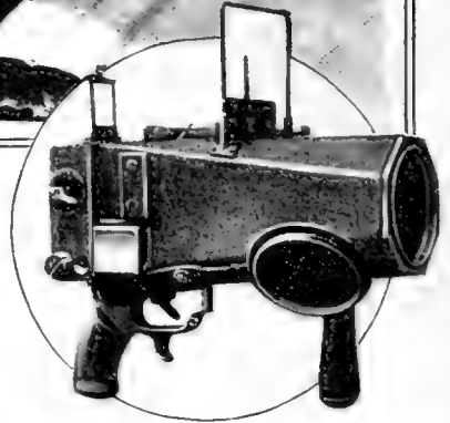
The Photographer in His Aeroplane Can Point the Pistol-Camera with Great Accuracy at the Object To Be Photographed. The Two Focusing Frames Take the Place of Sights on a Revolver. The Trigger Operates the Shutter
